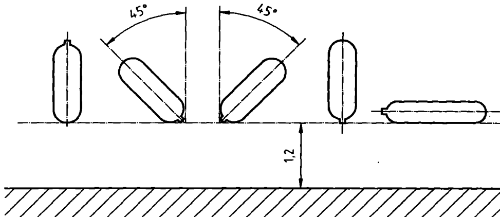
Figure 1 — Drop test
