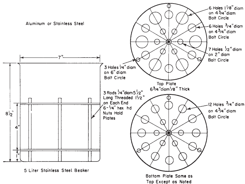
FIG. 2 Tube Holder (Aluminum or Stainless Steel) for Color-After-Heating Test
