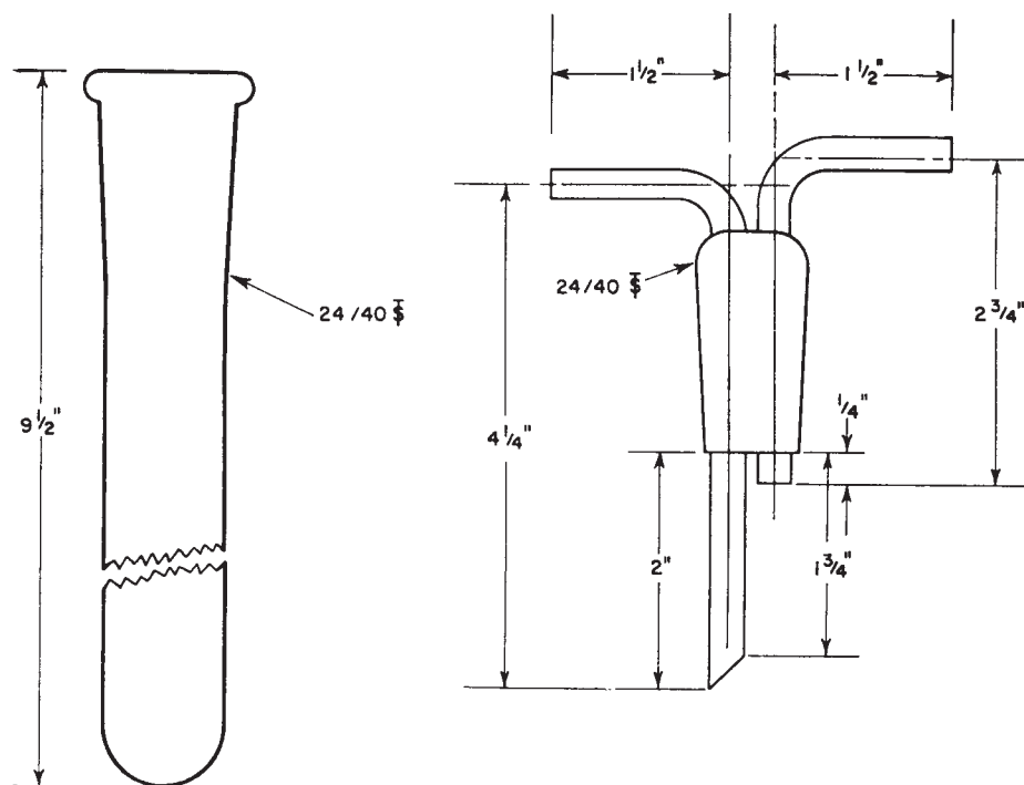
FIG. 1 Details of Color-After-Heating Tube
