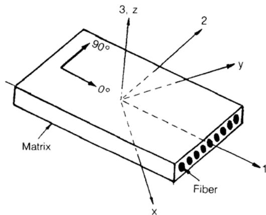
Figure 2 - Composite coordinate system
