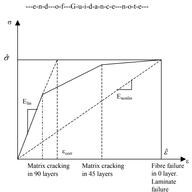
Figure 6 - Typical stress-strain relation for a laminate containing 0, 45 and 90 layers
