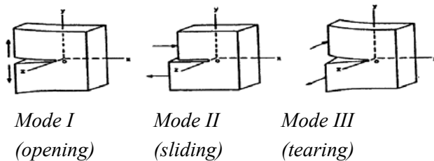
Figure 7- Inter-laminar failure modes
