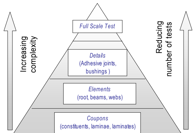
Figure 3- The Building Block Approach
