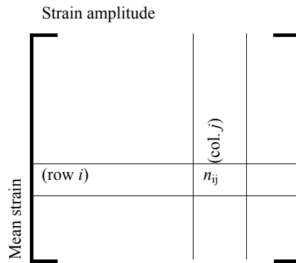
Figure 10 - Matrix representation of fatigue loads
