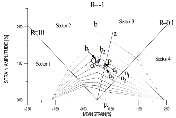
Figure 11 - A typical Constant Lifetime Diagram diagram.
