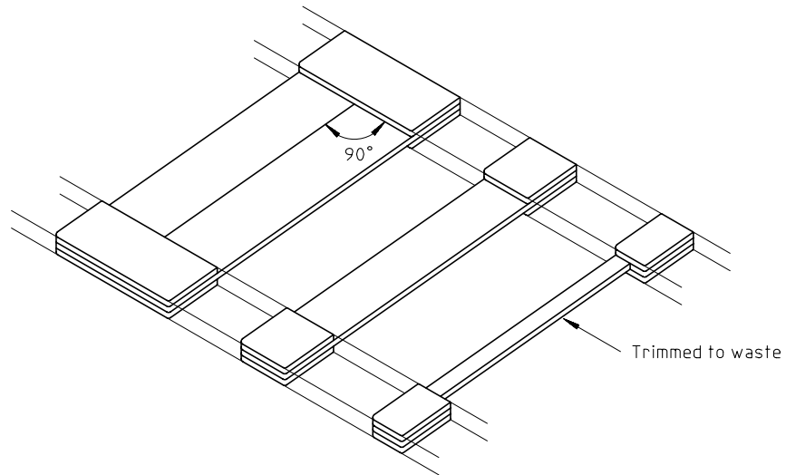
Figure A.1 — Tabbed panel for specimen preparation
